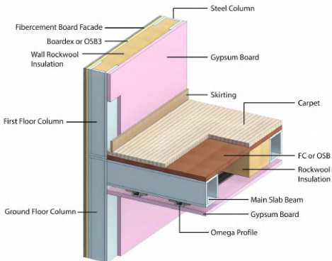
GET First Floor Slab Cross-Section
