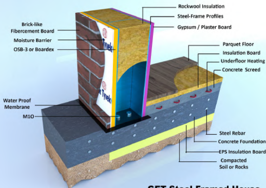
GET Steel-Framed House Exterior Wall and Ground Floor Cross-Sections
