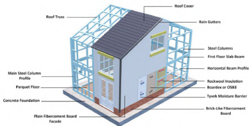
GET Design for Sheffield 108 m2 House
