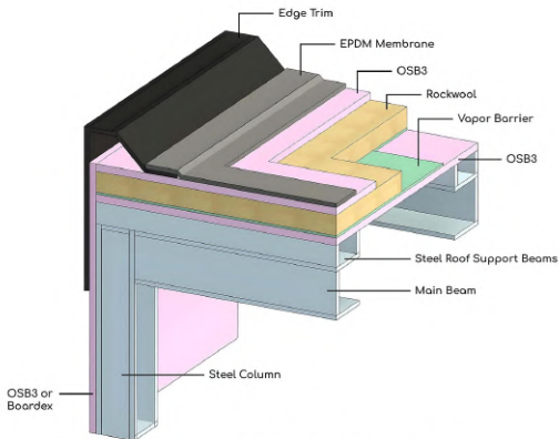
GET Flat Roof Cross-Section
