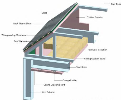
GET Sloped Roof Cross-Section
